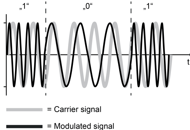
Figure 24: Frequency key shifting as a modulation method (FSK = F requency S hift K eying)
