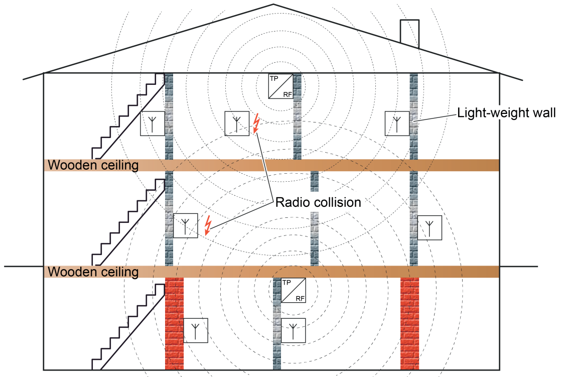
Figure 33: Building structure with two KNX RF lines, disadvantageous influence (example)
