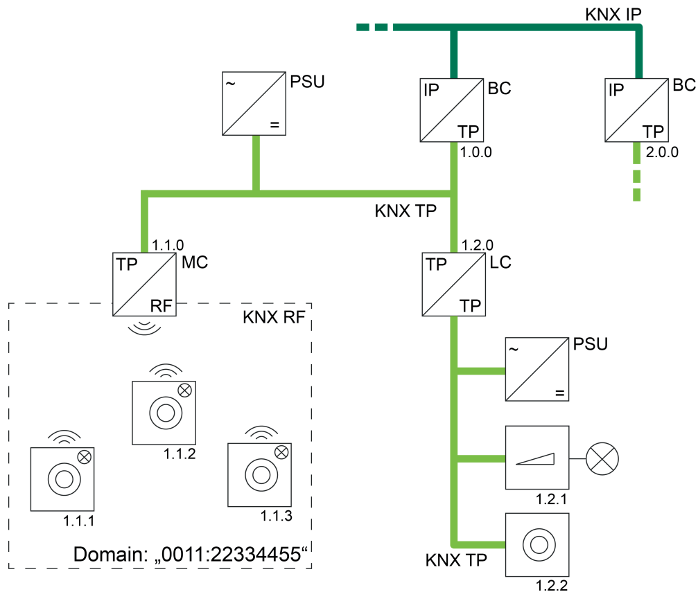
Figure 37: Example of a possible KNX topology with RF, TP and IP lines Media coupler as line coupler
