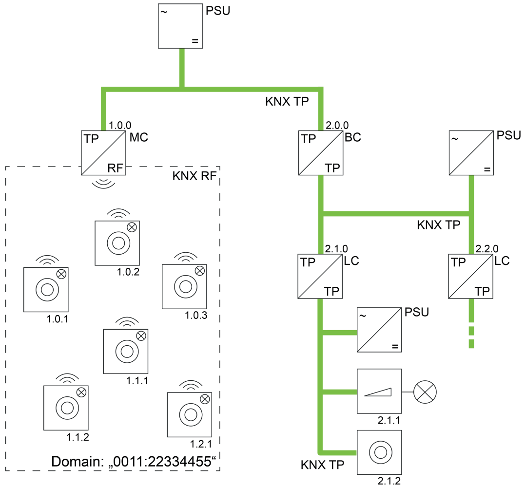
Figure 38: Example of a possible KNX topology with RF and TP lines Media coupler as backbone coupler
