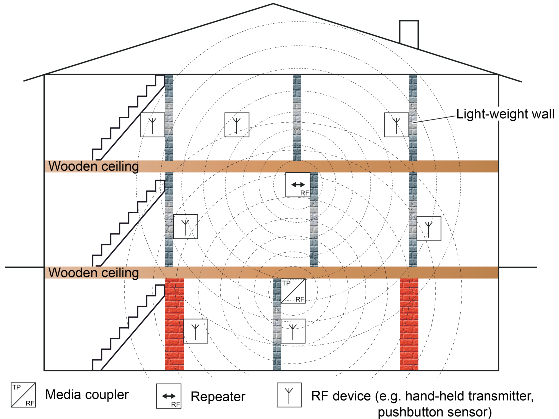
Figure 34: Building structure with one KNX RF line and repeater (example)
