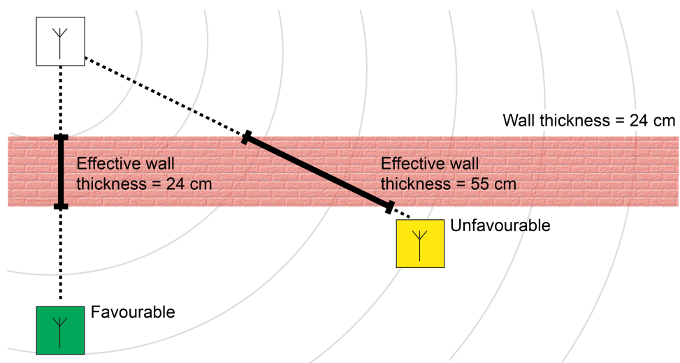
Figure 27: Attenuation through effective wall or ceiling thickness
