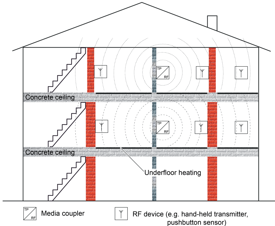
Figure 35: Building structure with two KNX RF lines, which do not influence each other negatively due to the building consistency (example)
