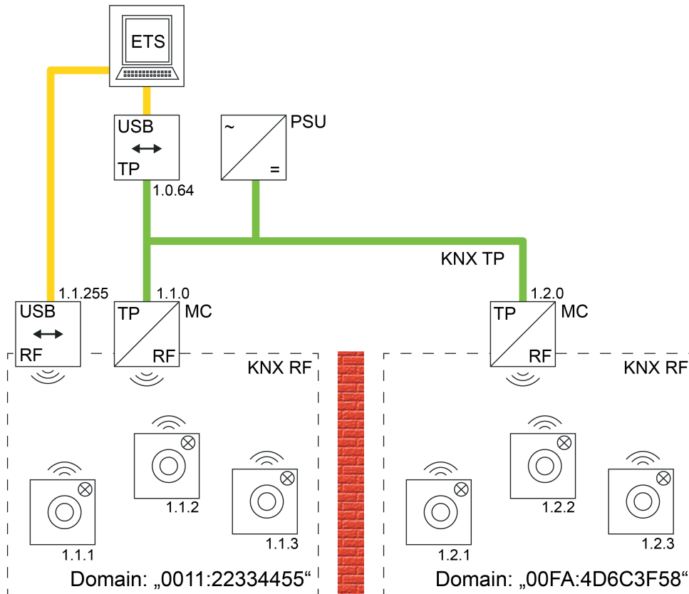
Figure 39: Example of a possible KNX topology with two RF lines and coupling via a TP main line (example)
