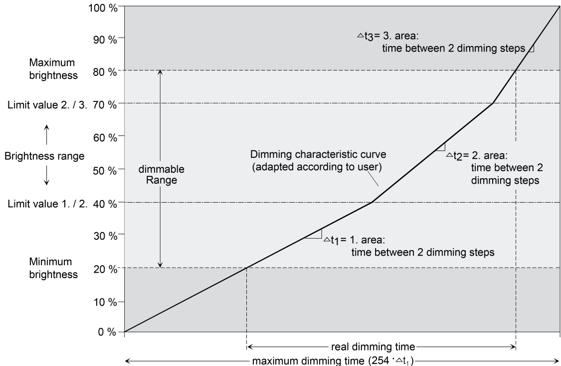
Figure 18: User-defined dimming characteristic as an example with minimum brightness and maximum brightness (example with 3 areas)
