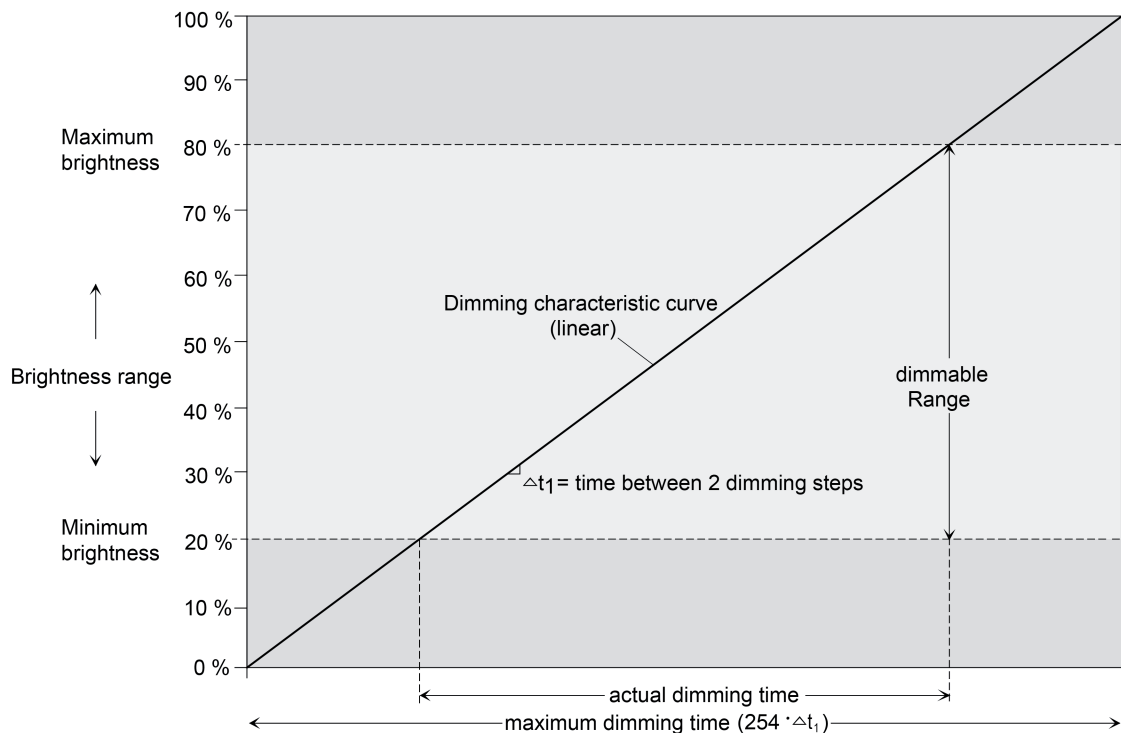
Figure 16: Linear characteristic dimming curve as an example with minimum brightness > 0 % and maximum brightness
