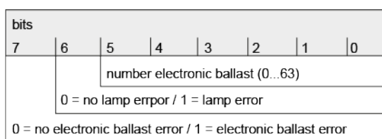
Figure 14: Telegram structure, 1-byte error status
