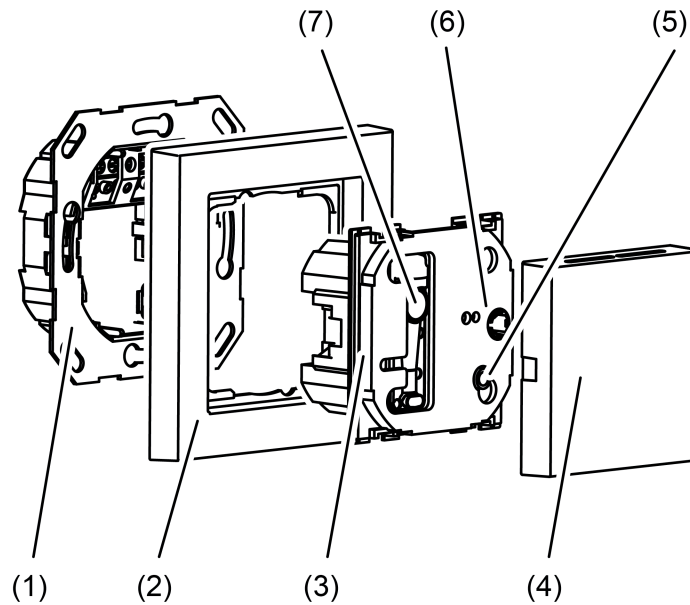
Figure 1: Device components CO 2 Sensor
