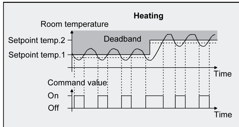
Figure 22: 2-point feedback control for mixed "Heating and cooling" mode with active heating mode.
