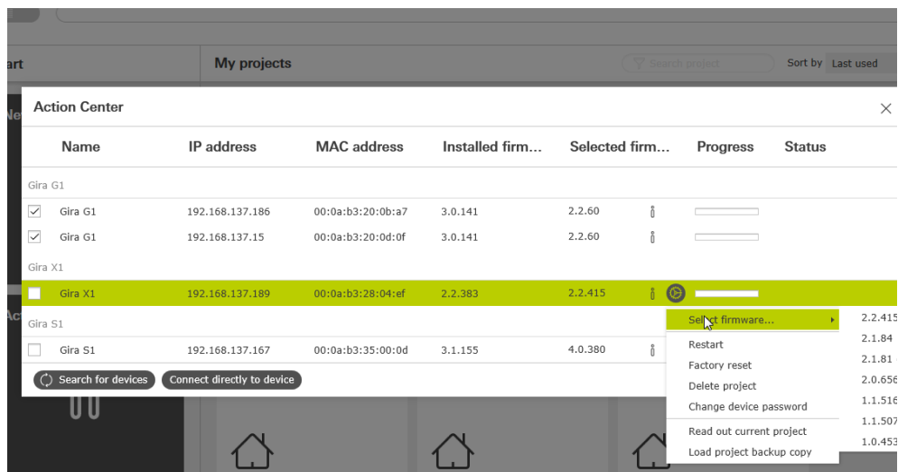
Figure 152 Gira Project Assistant Action Center
