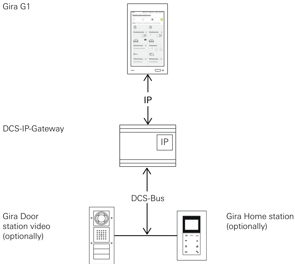
Figure 142 Gira G1 with DCS-IP gateway.
