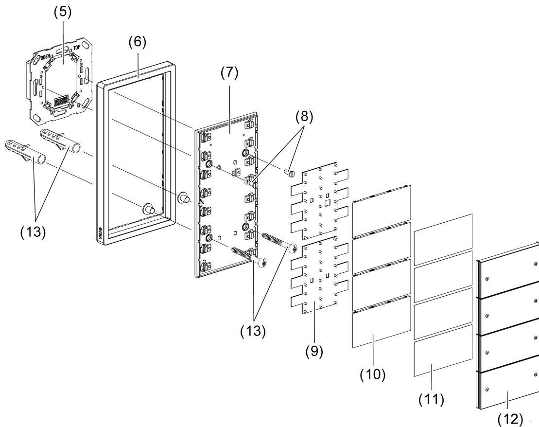
picture 3: Device fitting using the example of a push button sensor 3 comfort 4-gang F100 (doubled height)
