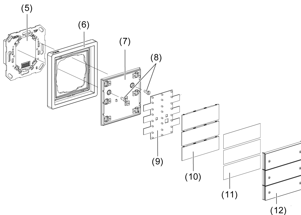
picture 2: Device fitting using the example of a push button sensor 3 comfort 3-gang F100
