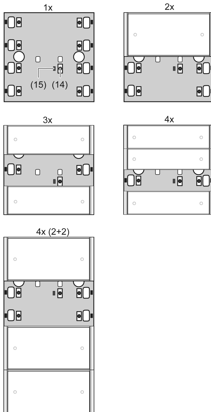
picture 4: Arrangement of the programming button and LED on the front of the device
