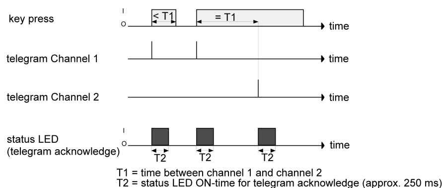
picture 17: Example for operation concept "Channel 1 and channel 2"
