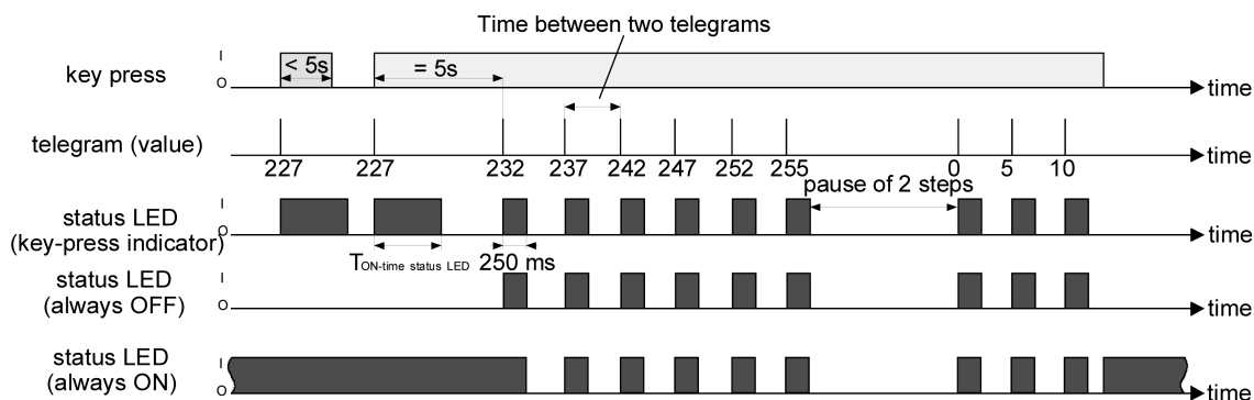
picture 15: Example of value adjustment with value range overflow
