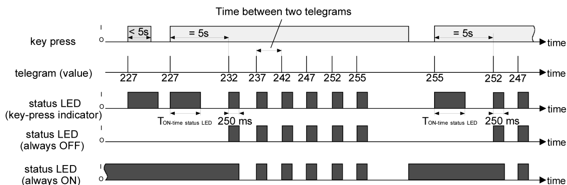
picture 14: Example of value adjustment without value range overflow
