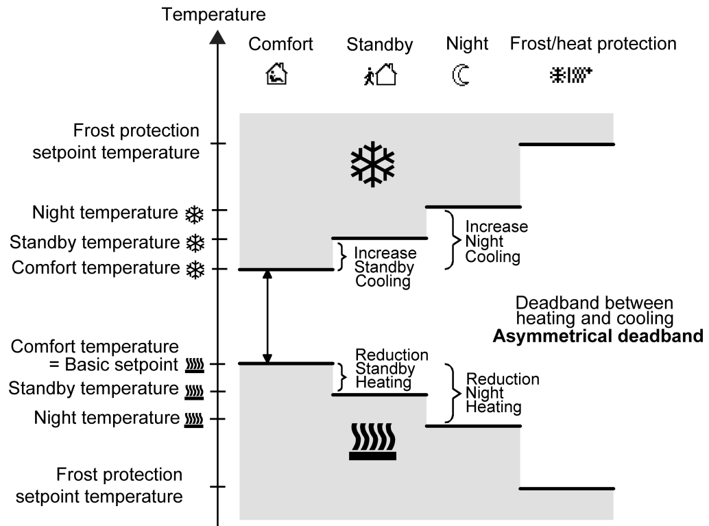
picture 47: Setpoint temperatures in the operating mode "Heating and cooling" with asymmetrical deadband
