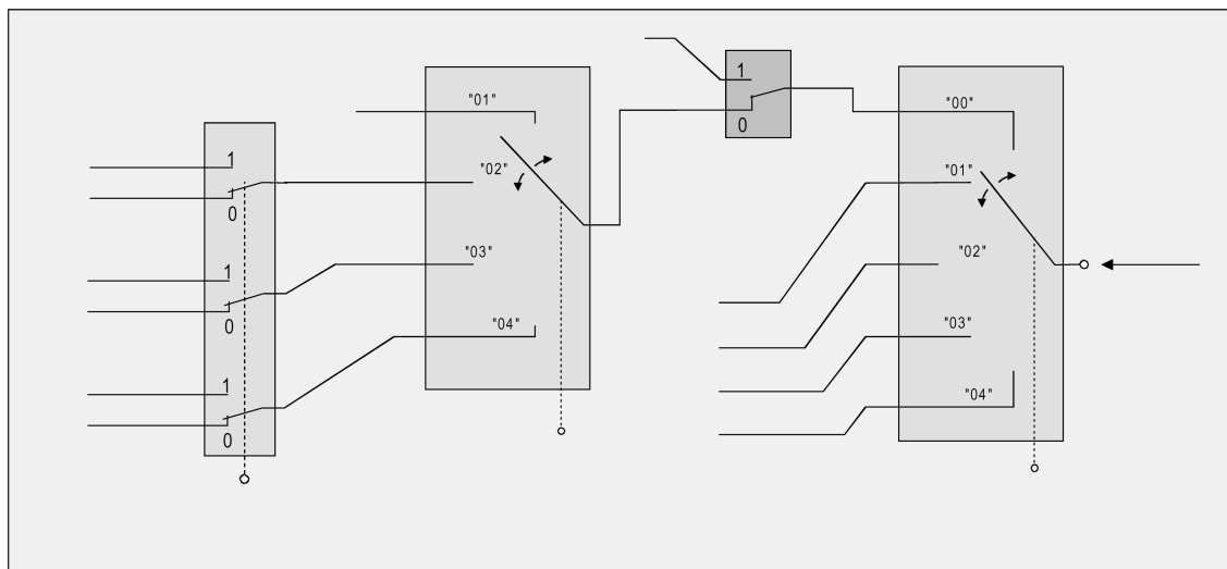
picture 40: Operating mode switchover through KONNEX object with presence button
