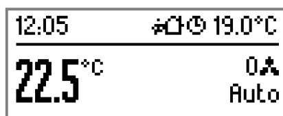
picture 6: Example of a basic display with two display areas (Time, setpoint temperature, room temperature, fan level display)
