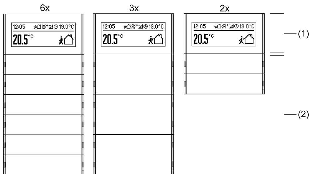
picture 5: Arrangement of the control surfaces on the front of the device
