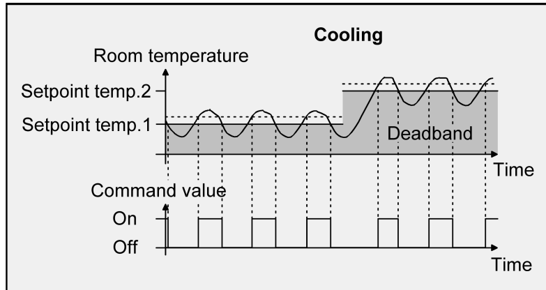
picture 35: 2-point feedback control for mixed "Heating and cooling" mode with active cooling operation.
