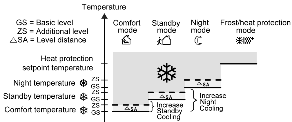
picture 45: Setpoint temperatures in the operating mode "Basic and additional cooling"
