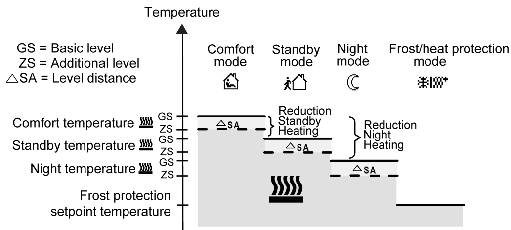
picture 43: Setpoint temperatures in the operating mode "Basic and additional heating"
