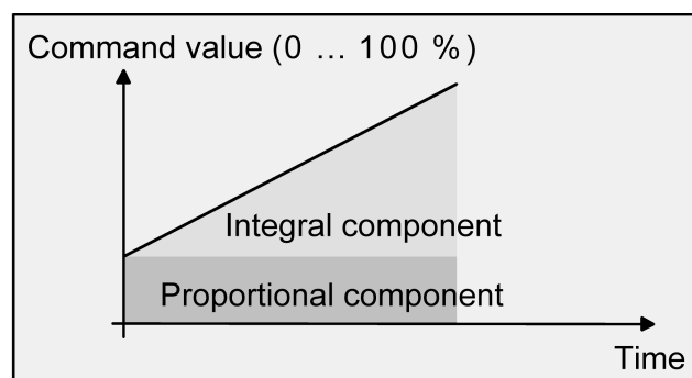
picture 30: Continuous PI control
