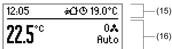
picture 50: Example of a basic display with two display areas (Time, setpoint temperature, room temperature, fan level display)
