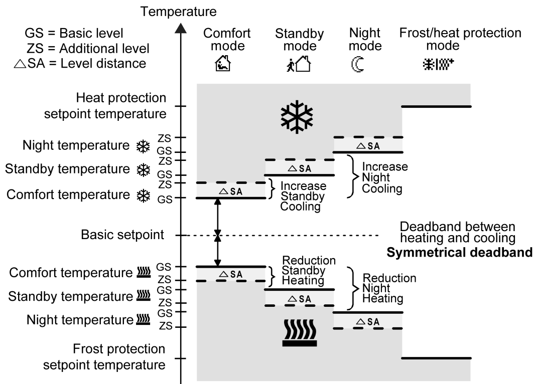
picture 48: Setpoint temperatures in the operating mode "Basic and additional heating and cooling" with symmetrical deadband
