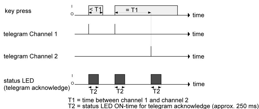
picture 28: Example for operation concept "Channel 1 and channel 2"
