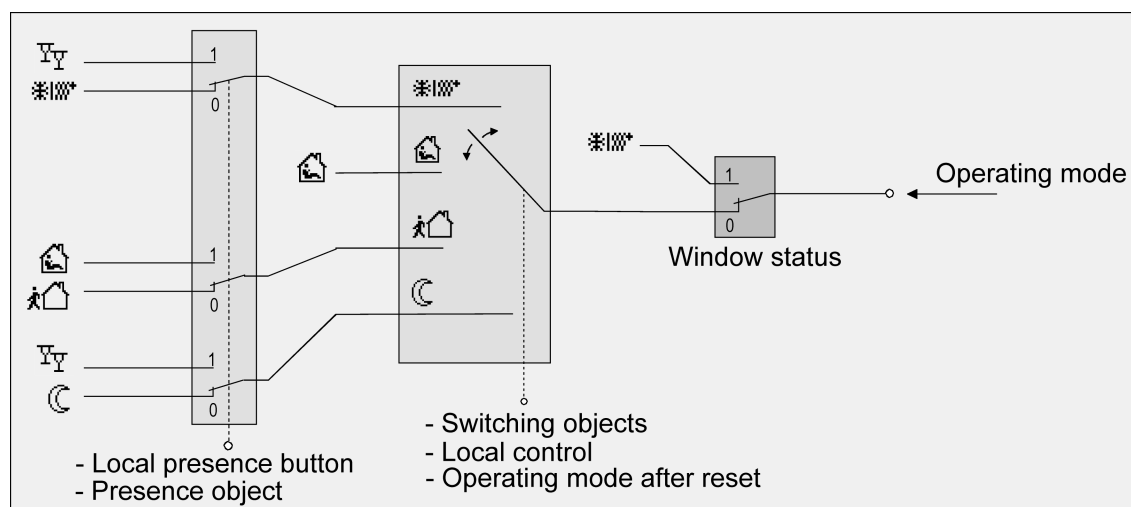
picture 38: Operating mode switchover through 4 x 1-bit objects with presence button
