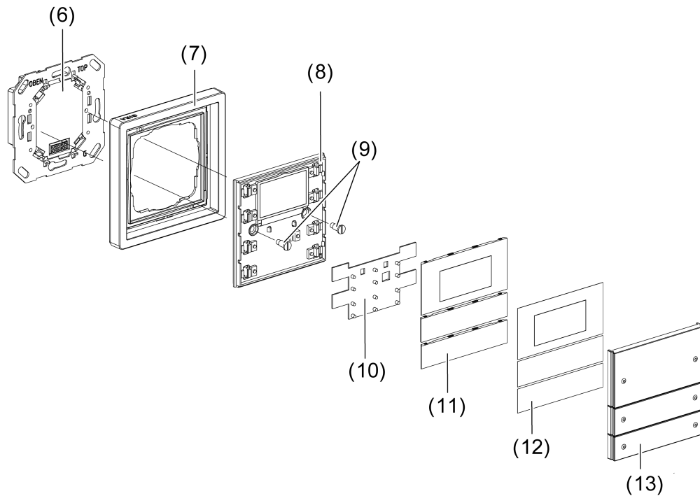
picture 2: Device fitting of a push button sensor 3 plus 2-gang F100
