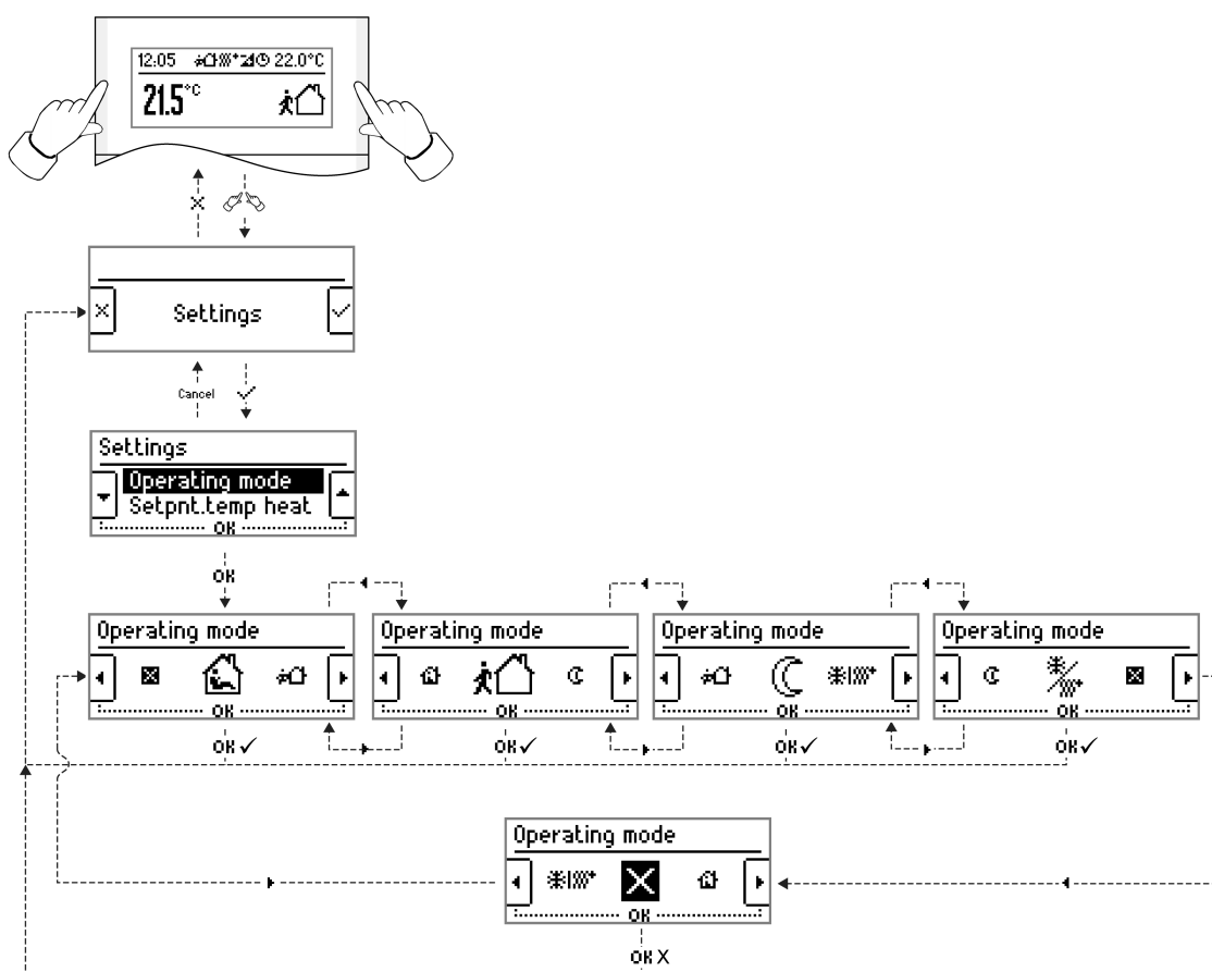
picture 11: Example for the submenu of the operating mode switchover
