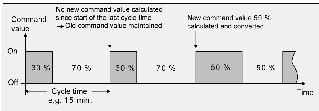
picture 31: Switching PI control
