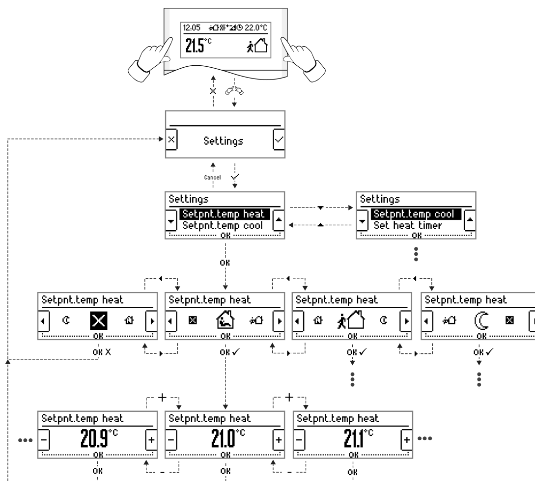
picture 12: Example of the submenu for setting setpoints for heating mode (applies similarly to cooling mode)
