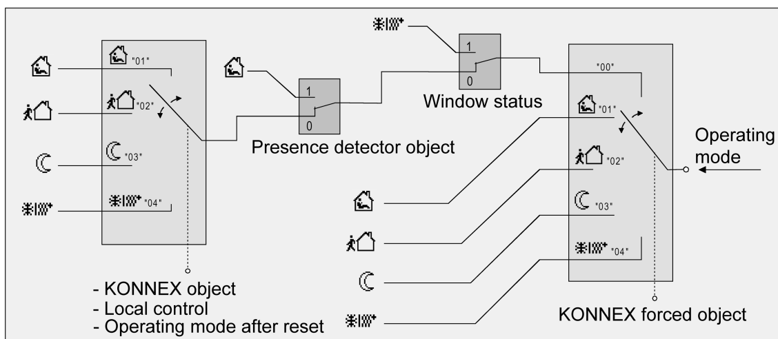
picture 41: Operating mode switchover through KONNEX object with motion detector
