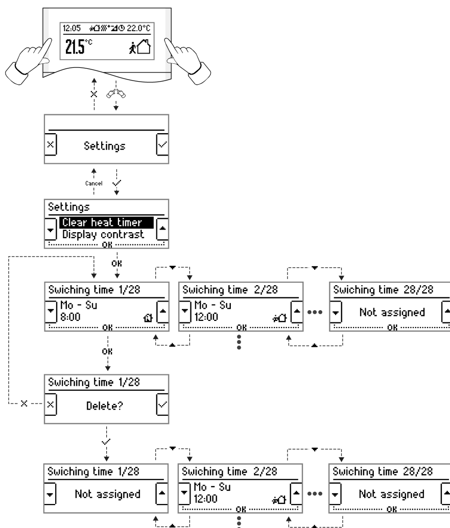
picture 14: Example of the submenu for deleting the switching times of the heating timer
