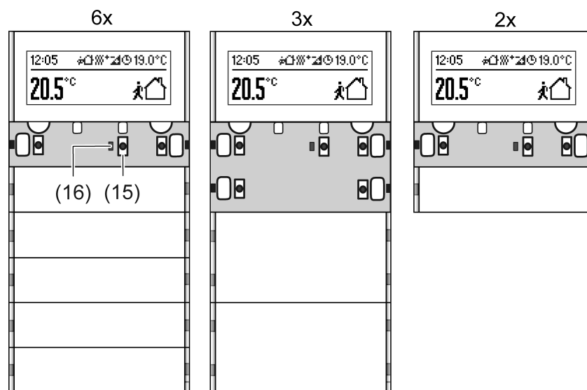
picture 4: Arrangement of the programming button and LED on the front of the device
