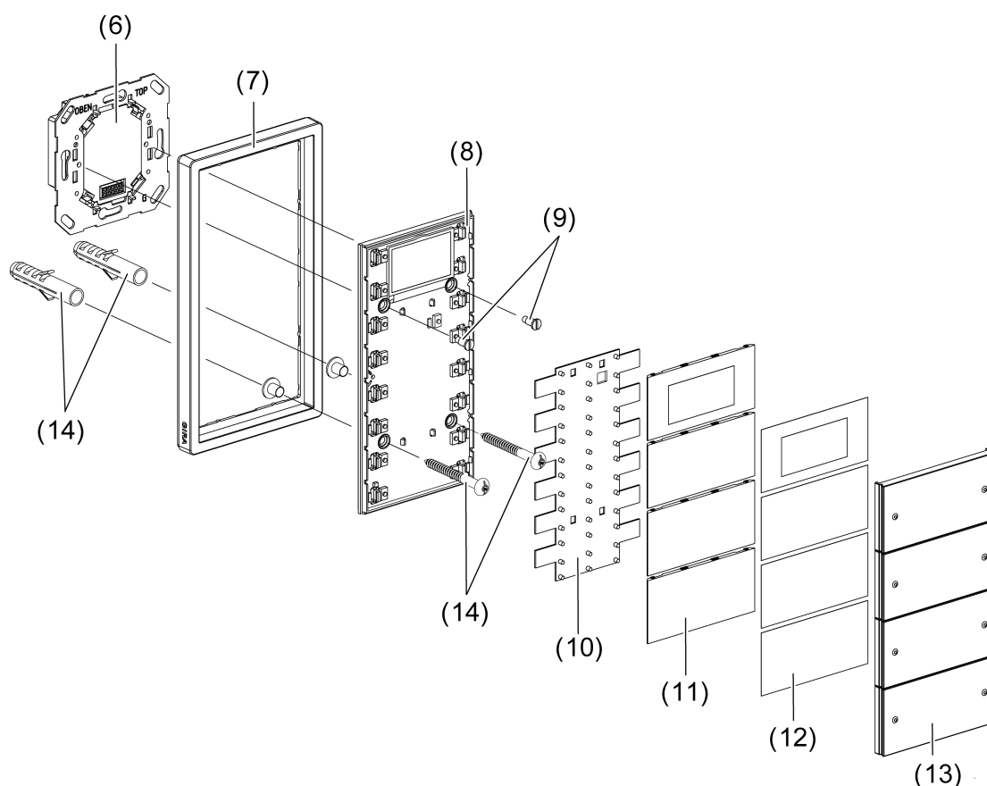
picture 3: Device fitting using the example of a push button sensor 3 plus 3-gang F100 (doubled height)
