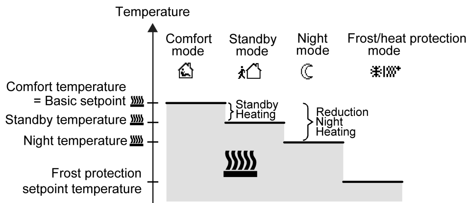
picture 42: Setpoint temperatures in the operating mode "Heating"
