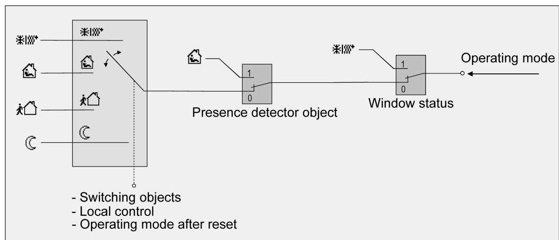
picture 39: Operating mode switchover through 4 x 1-bit objects with motion detector
