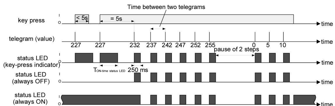
picture 26: Example of value adjustment with value range overflow
