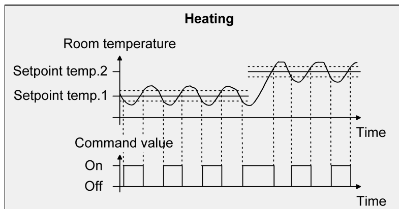
picture 32: 2-point feedback control for the single "Heating" operating mode
