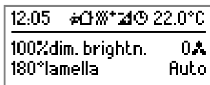
picture 56: Example of a 2-area display with 2-line value display incl. supplementary text. Line 1 brightness value, line 2 slat angle
