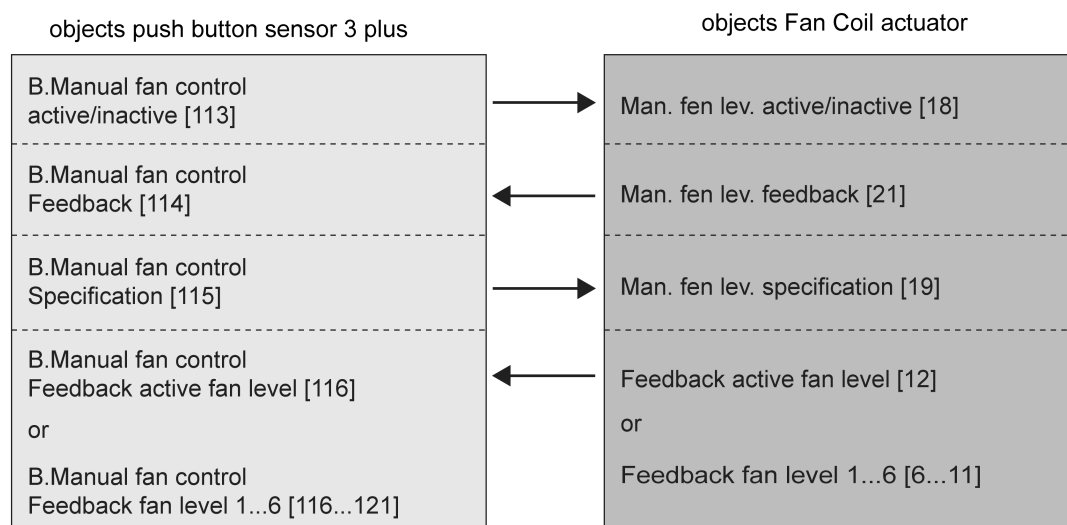
picture 64: Communication objects of the manual fan control (1-to-1 linking with objects of the fan coil actuator with the same functions)
