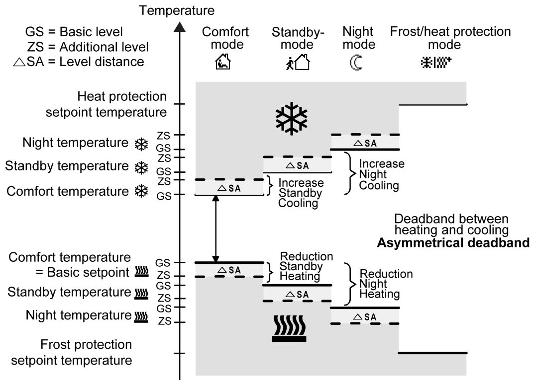
picture 49: Setpoint temperatures in the operating mode "Basic and additional heating and cooling" with asymmetrical deadband
