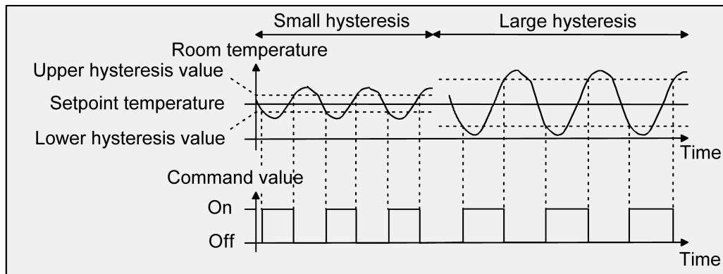
picture 37: Effects of the hysteresis on the switching behaviour of the command value of 2-point feedback control
