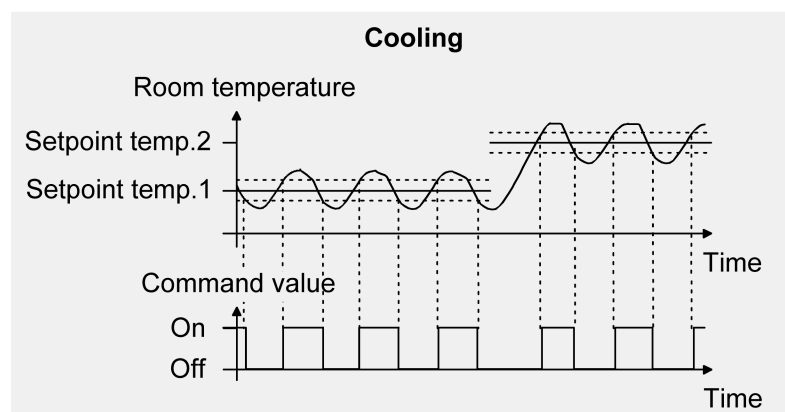
picture 33: 2-point feedback control for the single "Cooling" operating mode
