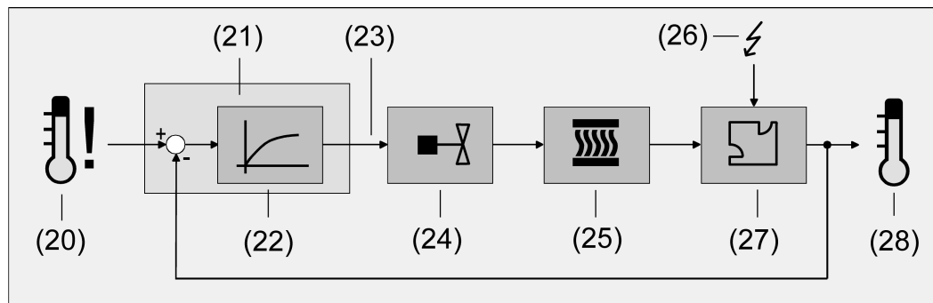
picture 29: Controlled system of single-room temperature control
