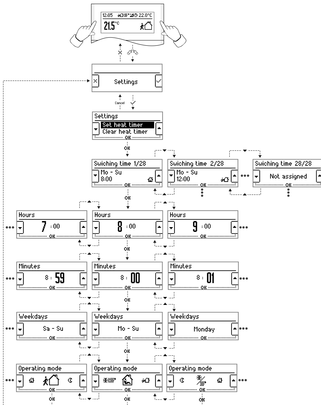
picture 13: Example of the submenu for setting the heating timer
