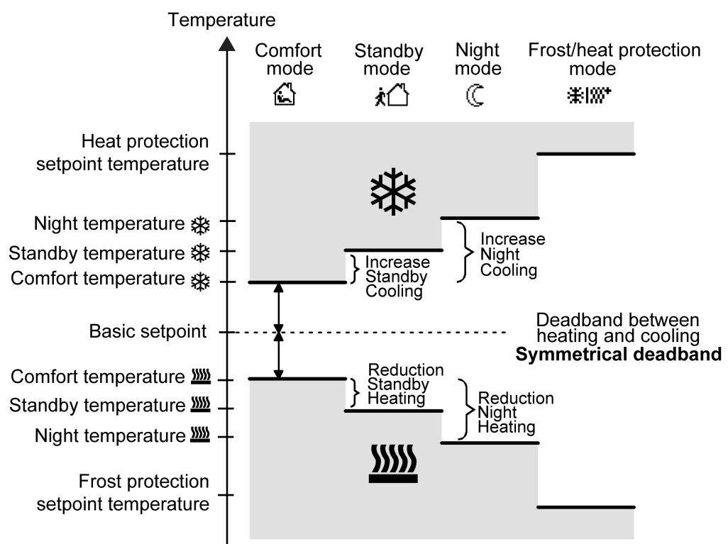
picture 46: Setpoint temperatures in the operating mode "Heating and cooling" with symmetrical deadband
