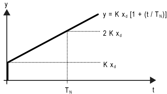
picture 36: Function of the command value of a PI control
