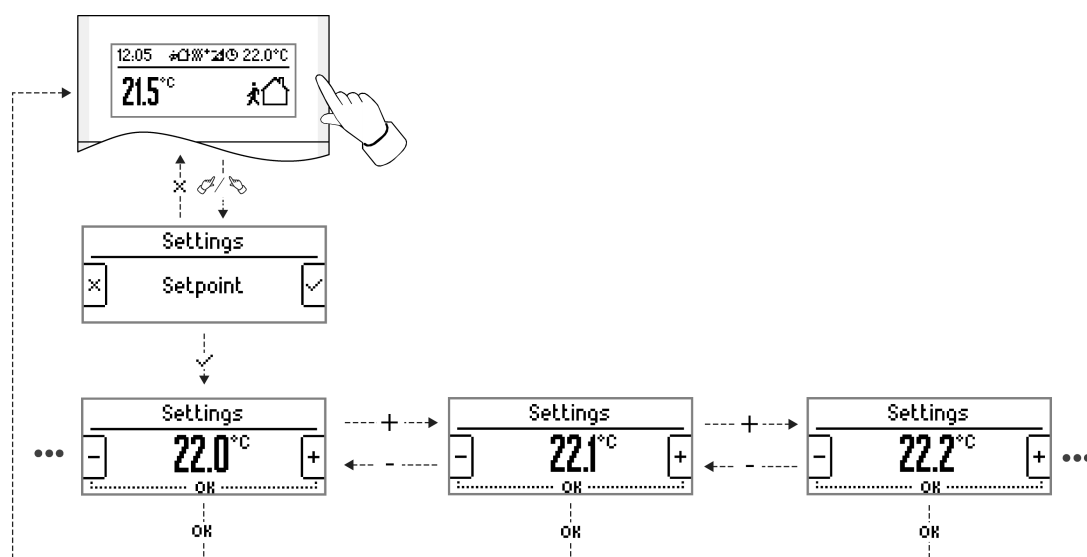
picture 8: Menu operation for setpoint shift Representation with absolute temperature value (not as bar graph)
